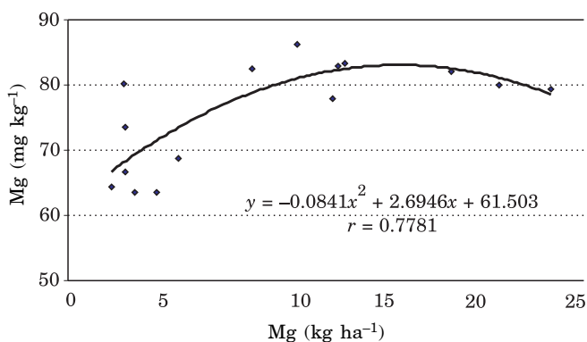
Fig. 2. Dependence of the concentration of available Mg in soil in \text{mg kg}^{-1} on the amount of the element accumulated in plant biomass in \text{kg ha}^{-1}
